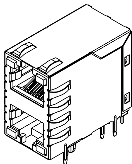
PN 6368011-1, 2, 3, 4, 5, 6, 8 & 1-6368011-1, 5 SCALE 2:1
