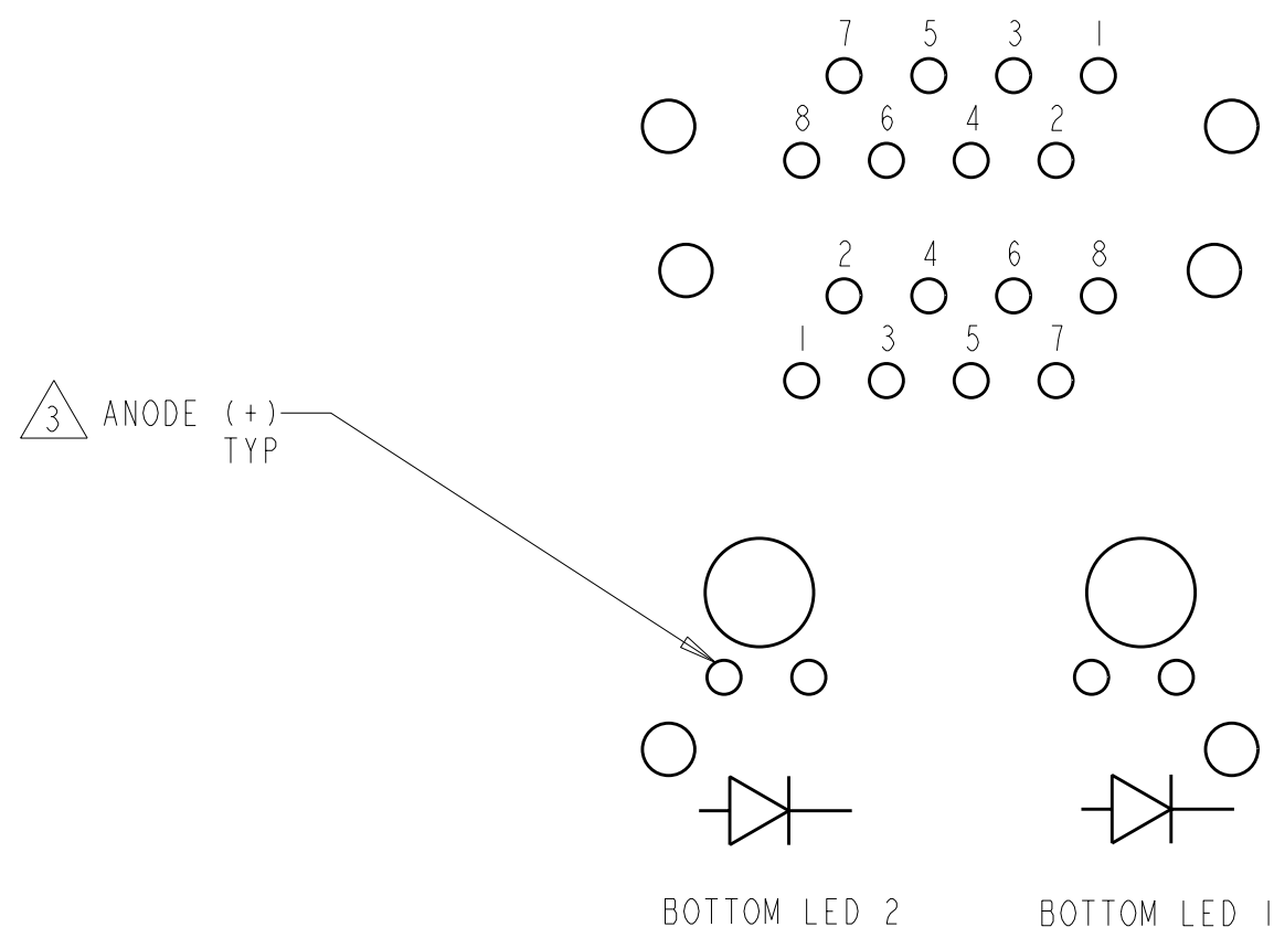
SCHEMATIC FOR 6368011-7, 1-6368011-3
