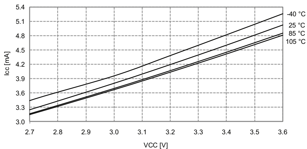
Figure 33-296. Idle Mode Current vs. V_{CC} f_{SYS} = 32\text{MHz} internal oscillator
