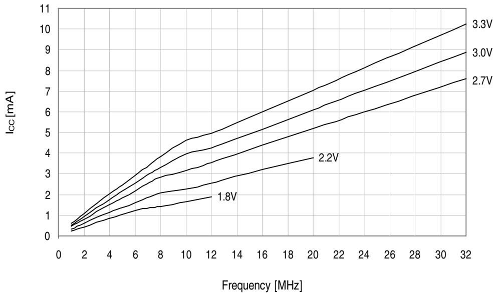
Figure 33-284.Active Supply Current vs. Frequency f_{SYS} = 1 - 32MHz external clock, T = 25^{\circ}C
