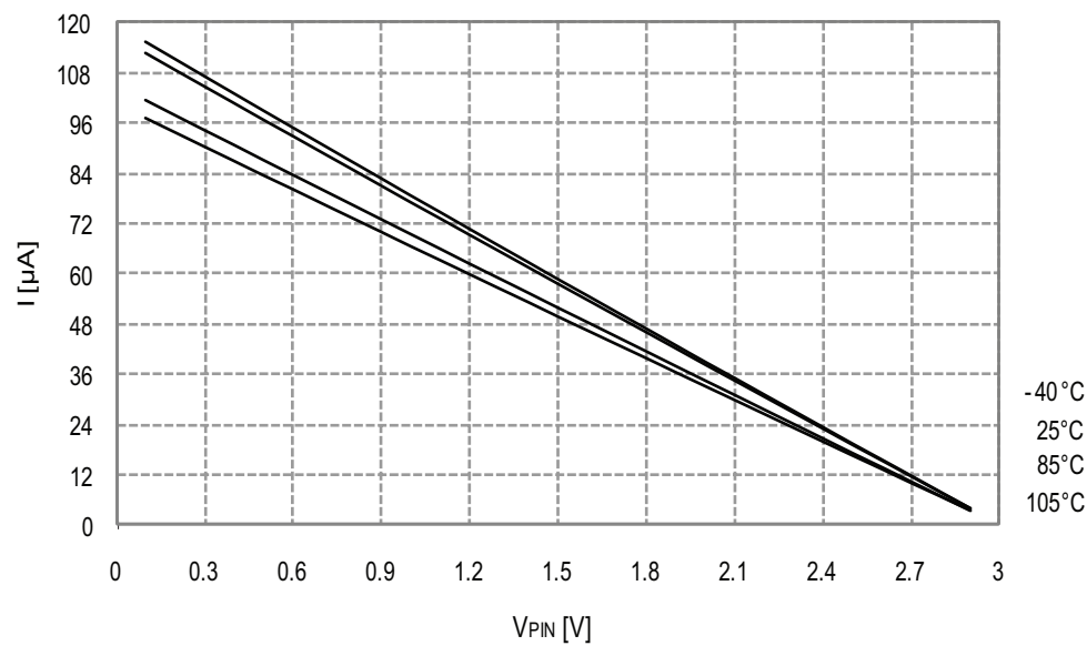
Figure 33-91. I/O Pin Pull-up Resistor Current vs. Input Voltage V_{CC} = 3.0V
