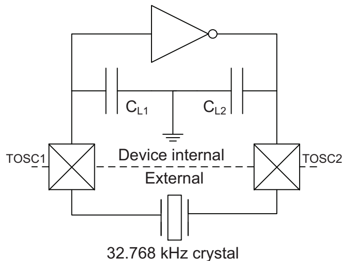
Figure 32-11.TOSC Input Capacitance
