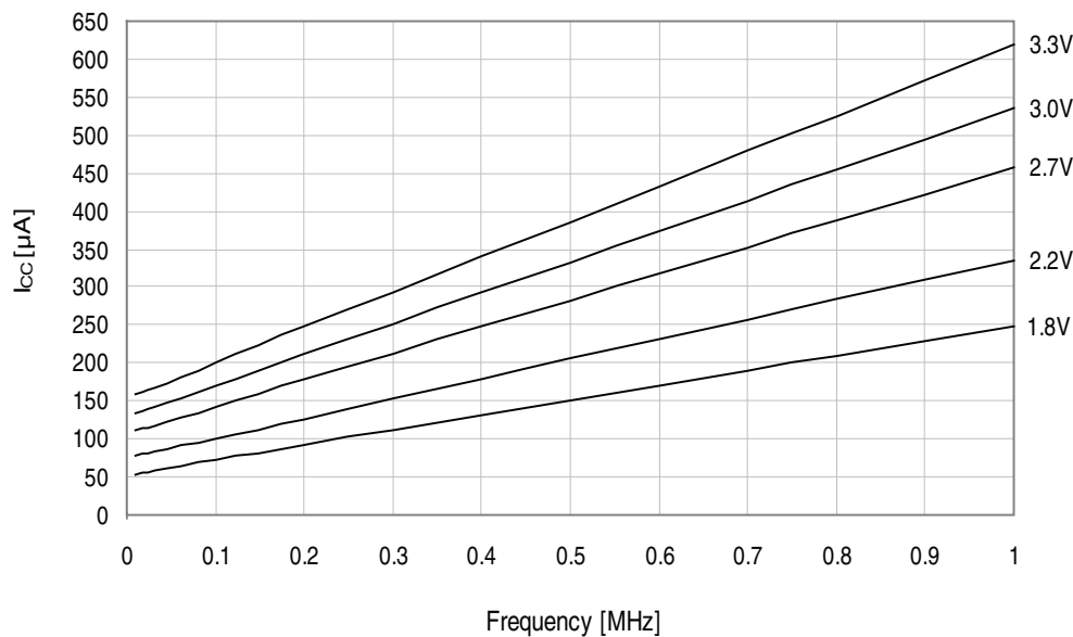
Figure 33-283.Active Supply Current vs. Frequency f_{SYS} = 0 - 1MHz external clock, T = 25^{\circ}C
