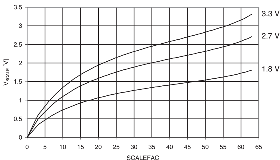
Figure 34-7. Analog Comparator Voltage Scaler vs. Scalefac T = 25^{\circ}\text{C}
