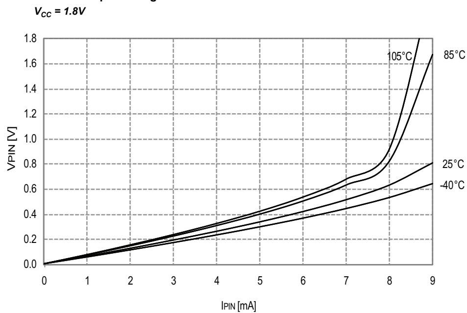
Figure 33-96. I/O Pin Output Voltage vs. Sink Current
