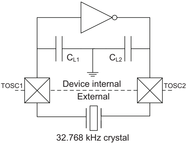
Figure 32-32. TOSC Input Capacitance
