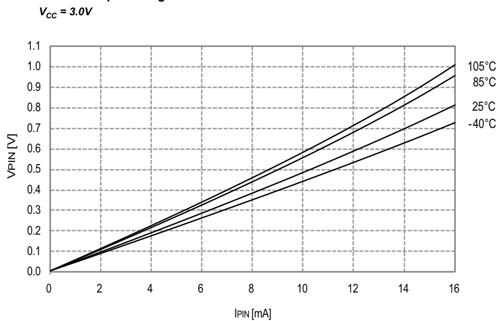
Figure 33-97. I/O Pin Output Voltage vs. Sink Current
