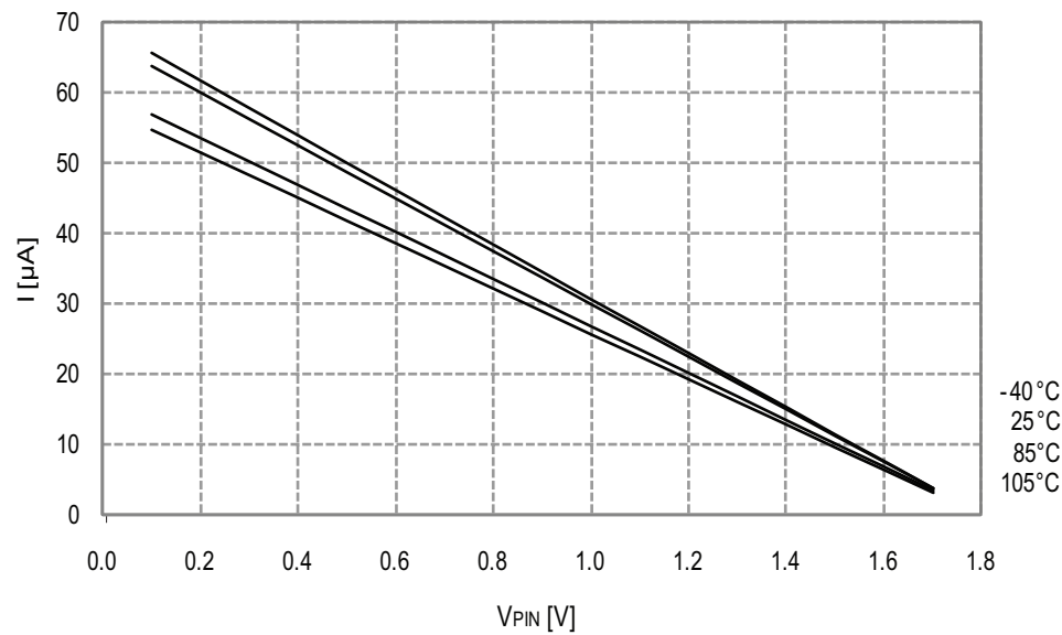
Figure 33-90. I/O Pin Pull-up Resistor Current vs. Input Voltage V_{CC} = 1.8V
