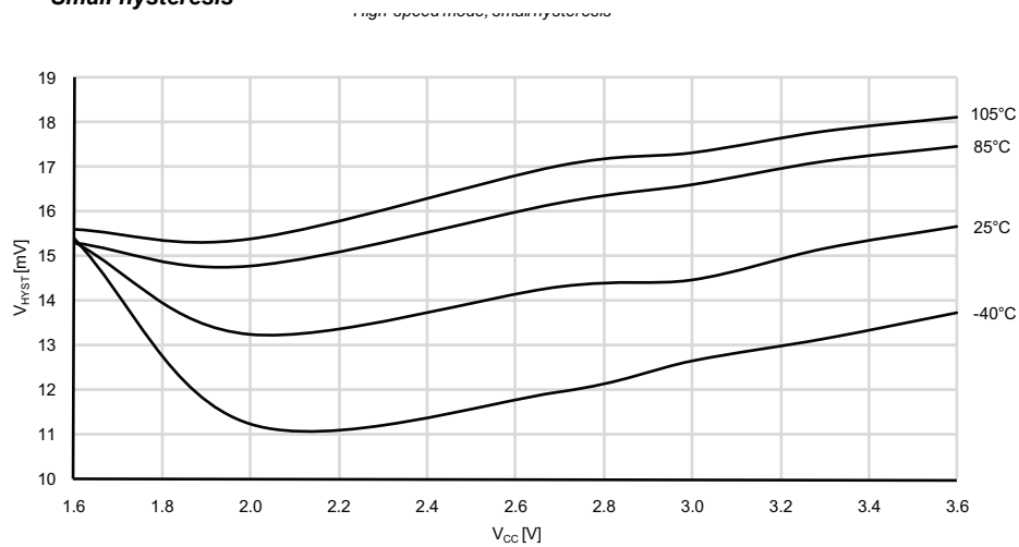
Figure 33-323. Analog Comparator Hysteresis vs. V_{CC} Small hysteresis
