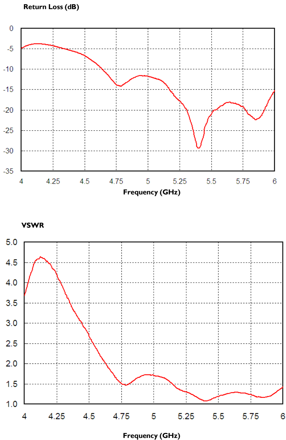
Fig. 3 Return loss & VSWR Measurement
