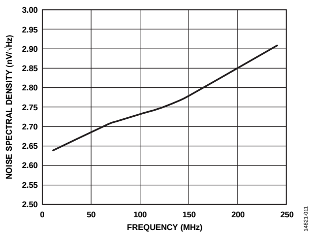
Figure 12. Noise Spectral Density (RTI) vs. Frequency ( R_L = 150\text{ }\Omega , 5 V Supply, A_V = 10\text{ dB} )
