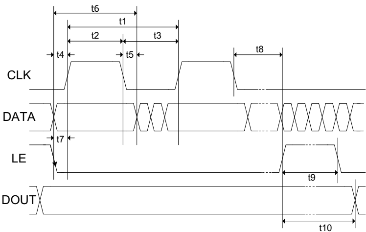
SPI Timing Diagram Specifications
