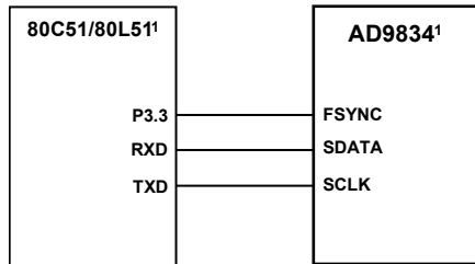
Figure 37. 80C51/80L51 to AD9834 Interface
