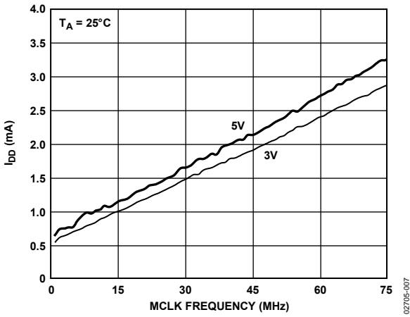
Figure 7. Typical Current Consumption ( I_{DD} ) vs. MCLK Frequency
