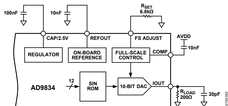
Figure 2. Test Circuit Used to Test the Specifications
