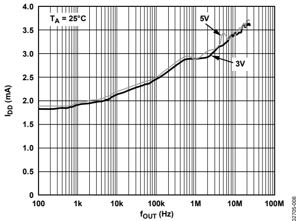
Figure 8. Typical I_{DD} vs. f_{OUT} for f_{MCLK} = 50\text{ MHz}
