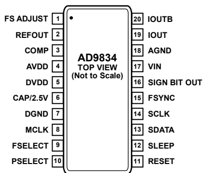
Figure 6. Pin Configuration
