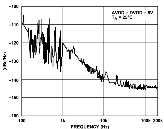
Figure 15. Output Phase Noise, f_{OUT} = 2 MHz, MCLK = 50 MHz
