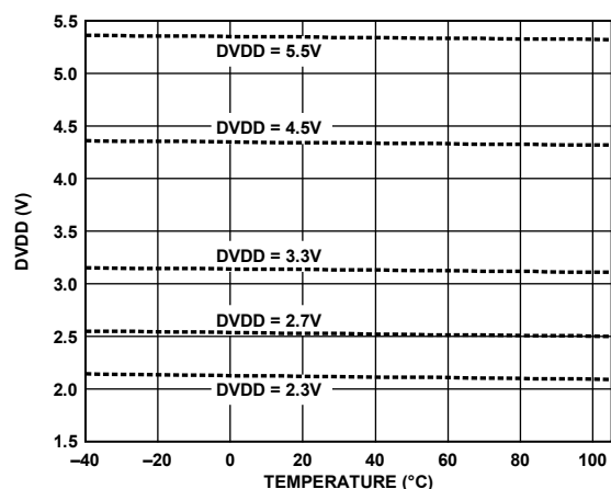
Figure 17. SIGN BIT OUT High Level, I_{SINK} = 1 mA
