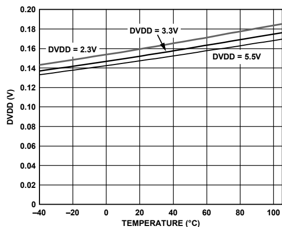
Figure 16. SIGN BIT OUT Low Level, I_{SINK} = 1 mA
