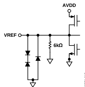
Figure 15. Equivalent VREF Circuit
