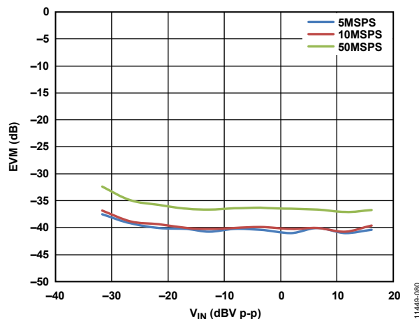
Figure 74. EVM vs. Input Voltage over Symbol Rates; Filter Bypass Mode, QPSK, Gain Code = 0000000, 1.5 V p-p Differential Output Level Maintained
