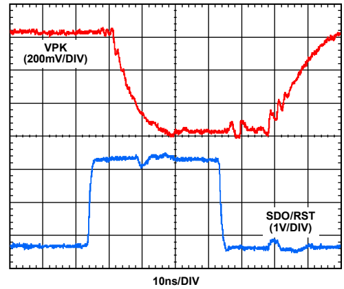
Figure 50. Peak Detector Hold Reset Time Domain Response
