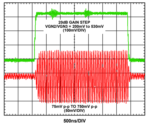
Figure 52. VGA2/VGA3 Gain Step Response; V_{GN1} = 0.5 V , -4 dBV RMS Input Signal Level, C17 and C32 = 100 pF
