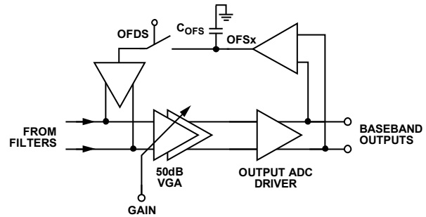
Figure 71. Offset Compensation Loop Operates Around the VGA and Output Buffer
