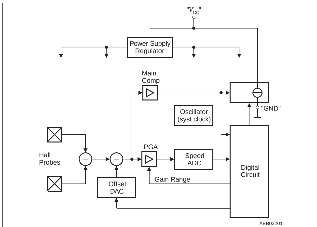
Figure 2 Block Diagram
