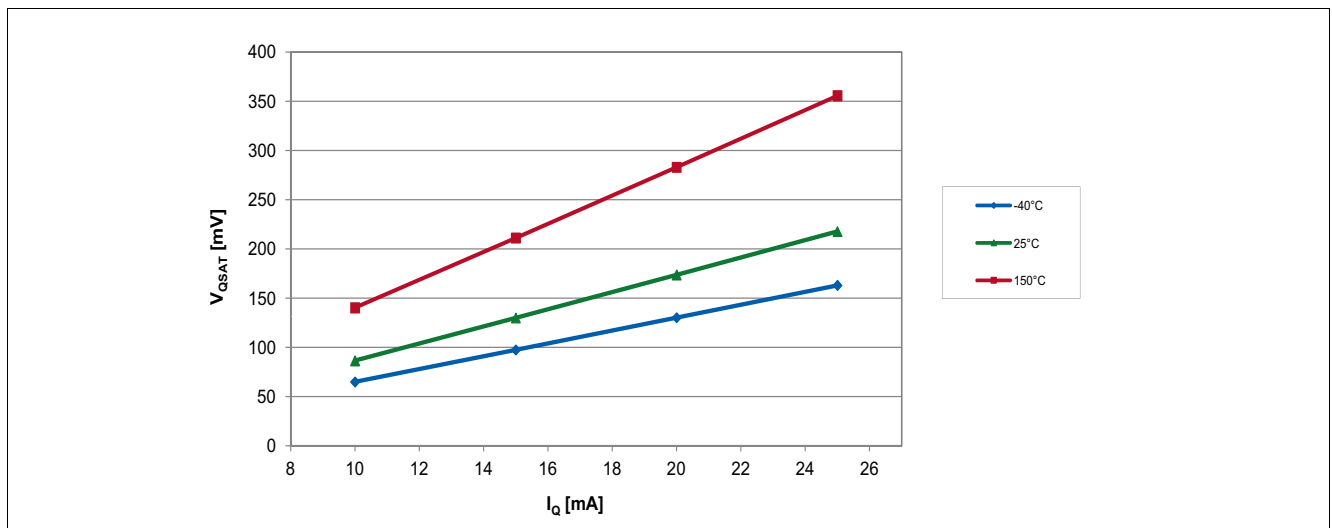
Figure 6-13 Saturation Voltage of the TLE4961-1L over Output Current
