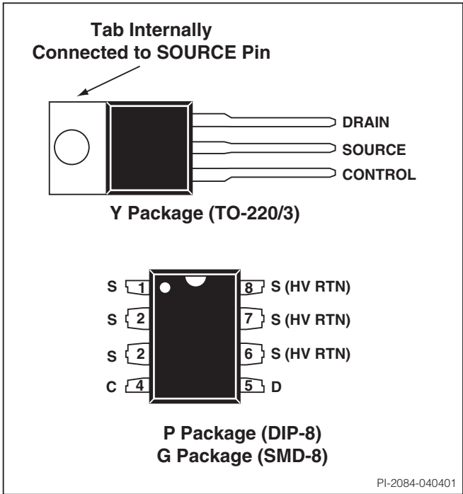
Figure 3. Pin Configuration.
