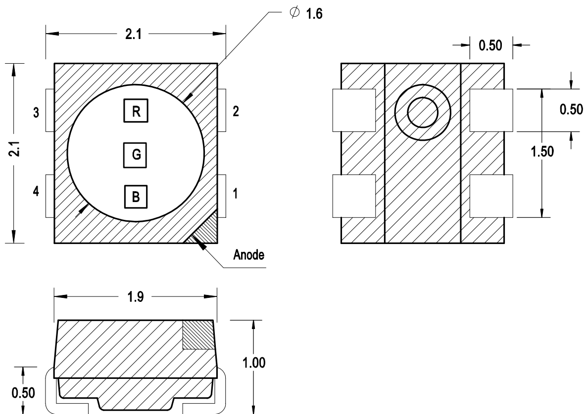
Figure 1: Package Drawing
