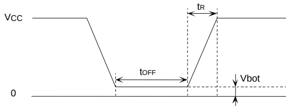
Figure 52. Rise waveform diagram
