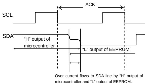
Figure 46. Input / output collision timing
