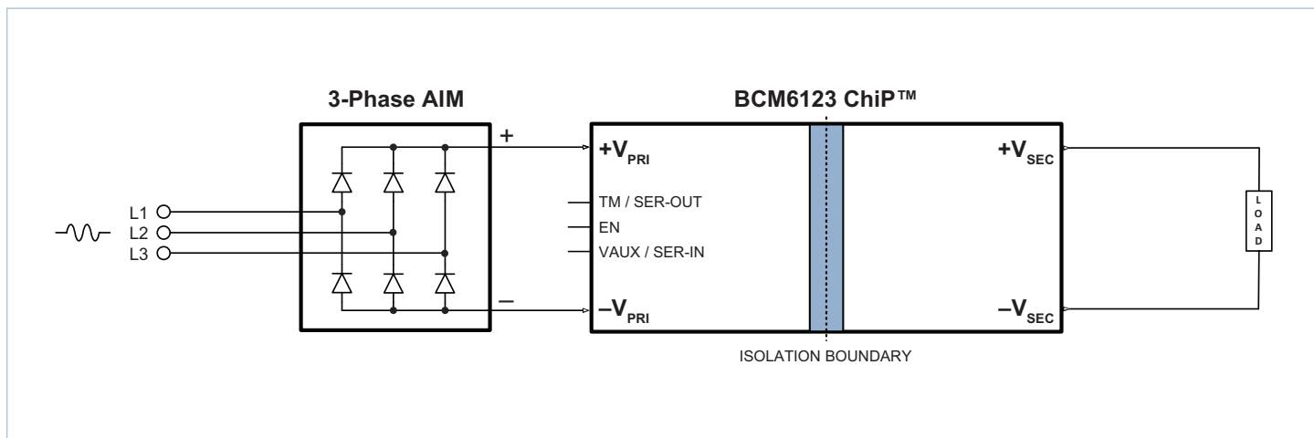
3-phase AC to point-of-load (3-phase AIM™ + BCM6123xD1E13A3yzz)
