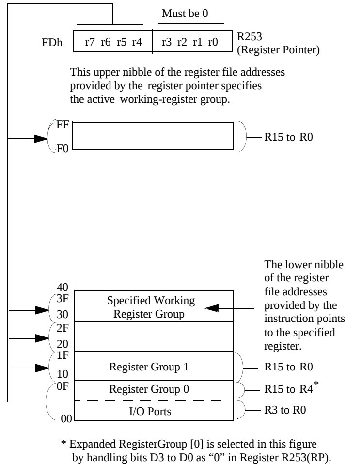
Figure 15. Register Pointer
