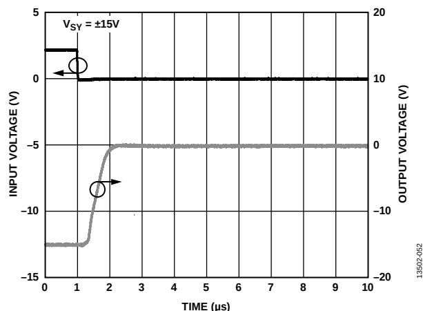
Figure 51. Negative Overload Recovery, A_V = -10 , V_{SY} = \pm 15\text{ V}
