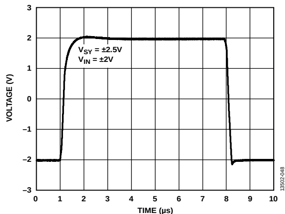
Figure 47. Large Signal Transient Response, V_{SY} = \pm 2.5\text{ V}
