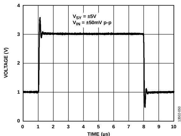
Figure 49. Small Signal Transient Response, V_{SY} = \pm 5\text{ V}
