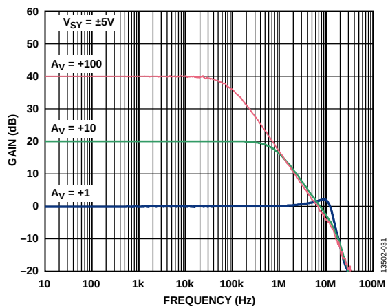
Figure 30. Closed-Loop Gain vs. Frequency, V_{SV} = \pm 5V
