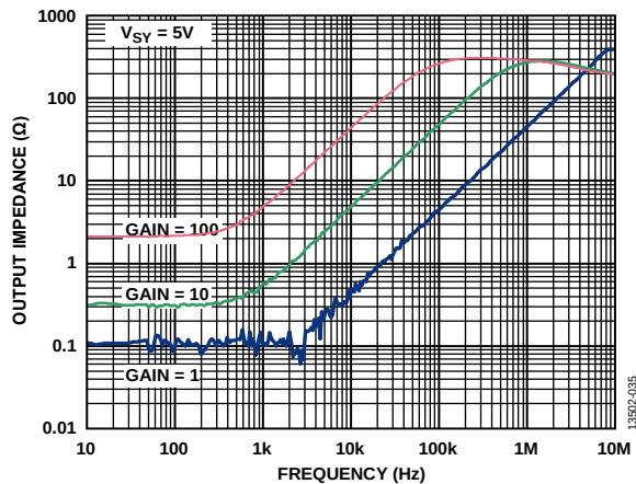
Figure 34. Output Impedance vs. Frequency, V_{SV} = 5V
