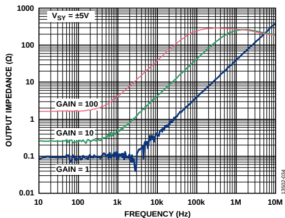
Figure 33. Output Impedance vs. Frequency, V_{SV} = \pm 5V
