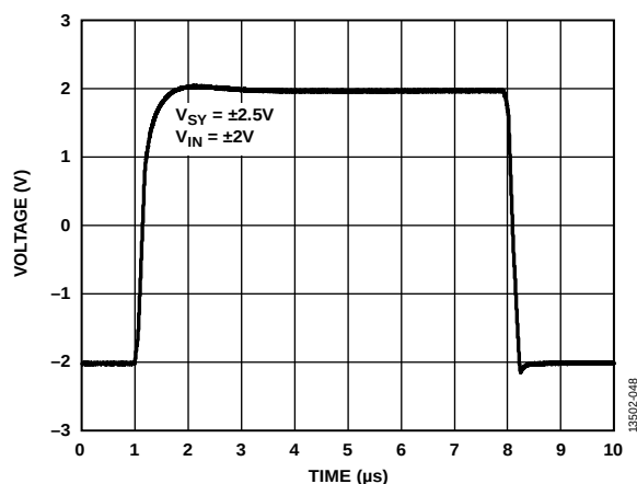
Figure 47. Large Signal Transient Response, V_{SV} = \pm 2.5\text{ V}
