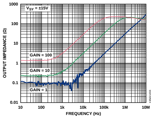
Figure 32. Output Impedance vs. Frequency, V_{SV} = \pm 15V
