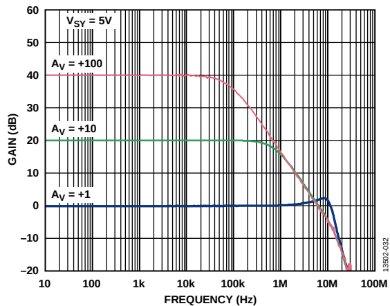
Figure 31. Closed-Loop Gain vs. Frequency, V_{SV} = 5V
