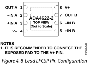
Figure 4. 8-Lead LFCSP Pin Configuration
