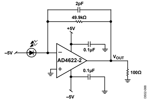
Figure 87. Photodiode Preamplifier
