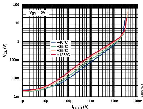
Figure 21. Output Voltage Low ( V_{OL} ) to Supply Rail vs. Load Current ( I_{LOAD} ) over Temperature, V_{SY} = 5V
