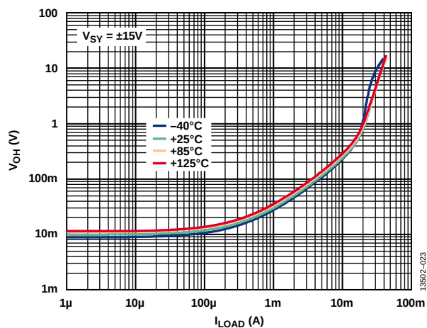
Figure 22. Output Voltage High ( V_{OH} ) to Supply Rail vs. Load Current ( I_{LOAD} ) over Temperature, V_{SY} = \pm 15V
