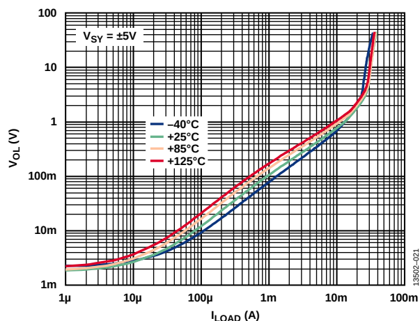
Figure 20. Output Voltage Low ( V_{OL} ) to Supply Rail vs. Load Current ( I_{LOAD} ) over Temperature, V_{SY} = \pm 5V
