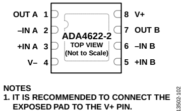
Figure 4. 8-Lead LFCSP Pin Configuration
