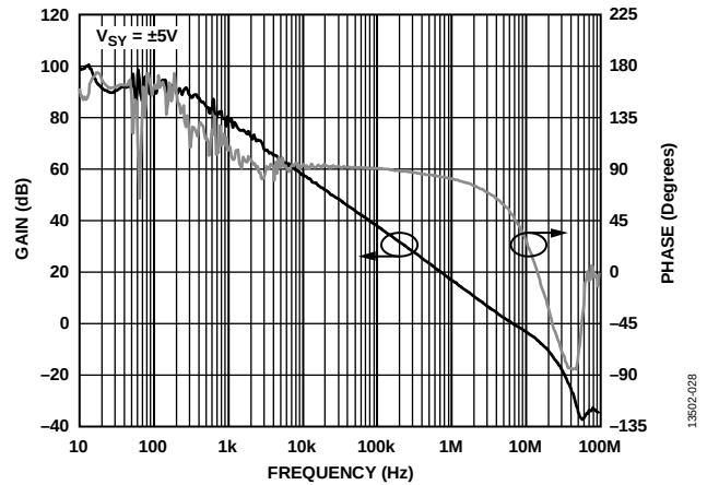
Figure 27. Open-Loop Gain and Phase vs. Frequency, V_{SY} = \pm 5 V
