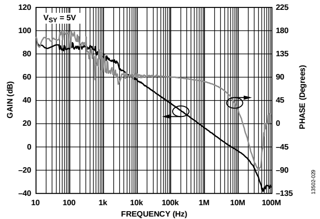
Figure 28. Open-Loop Gain and Phase vs. Frequency, V_{SY} = 5 V
