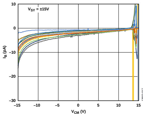
Figure 16. Input Bias Current ( I_B ) vs. Input Common-Mode Voltage ( V_{CM} ), V_{SY} = \pm 15\text{ V}
