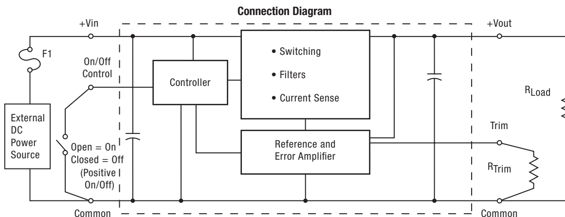
Figure 1. OKY-T/3, -T/5
