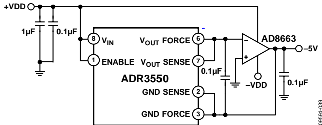
Figure 39. ADR3550 Negative Reference
