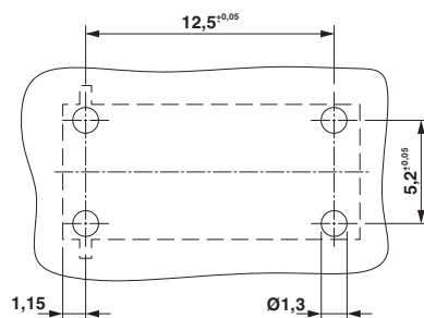
Drilling diagram
