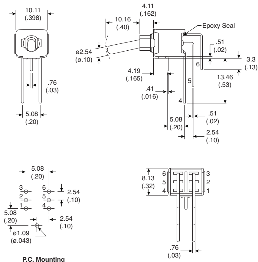
P.C. Mounting
