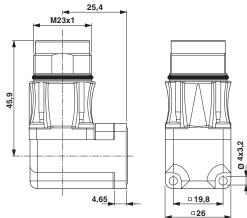
Dimensioned drawing
