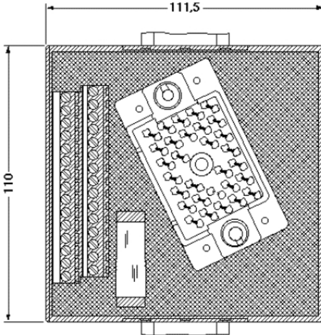
Dimensioned drawing
