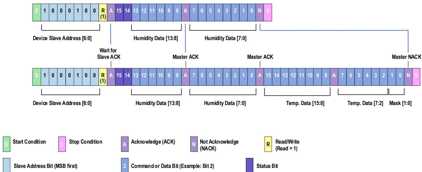
Figure 16. Data Fetch
