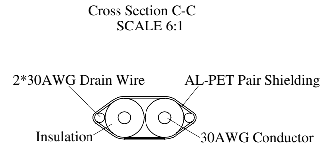
Parallel Pair Unit SCALE 20:1
