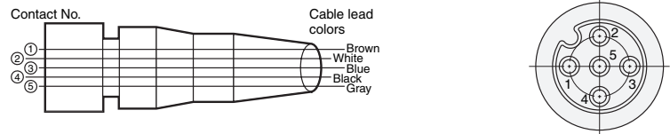
Wiring Diagram
