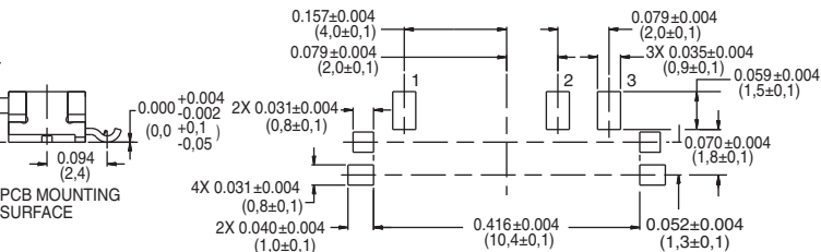
JSM05000SAQN SP3T Surface Mount Momentary both sides
