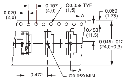
CARRIER TAPE
