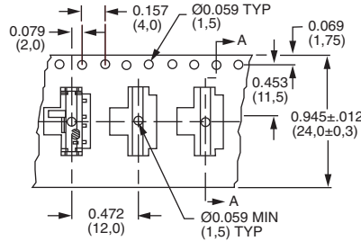
CARRIER TAPE
