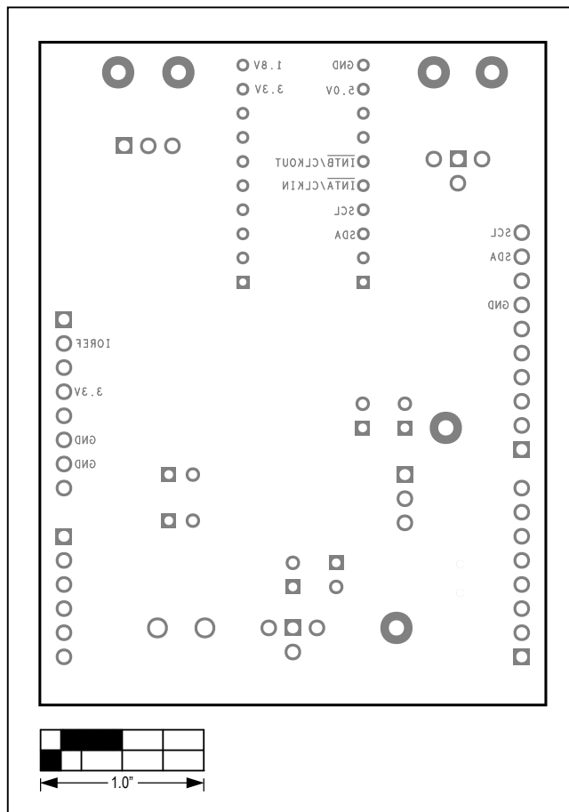
MAX31341 Shield EV Kit—PCB Bottom Silkscreen
