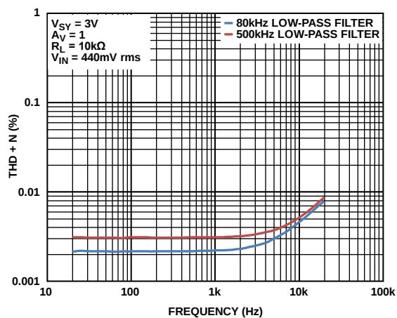
Figure 62. THD + N vs. Frequency
