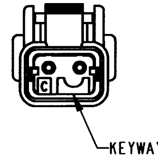
DTMH06-2SC -C- KEY TPA COLOR: GREEN
