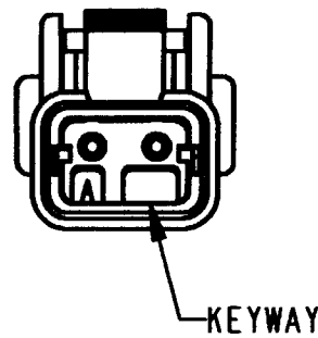
DTMH06-2SA -A- KEY TPA COLOR: GREY
