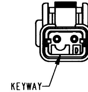
DTMH06-2SD -D- KEY TPA COLOR: BROWN
