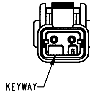
DTMH06-2SB -B- KEY TPA COLOR: BLACK
