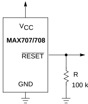
Figure 14. Ensuring RESET Valid to V_{CC} = 0 V
