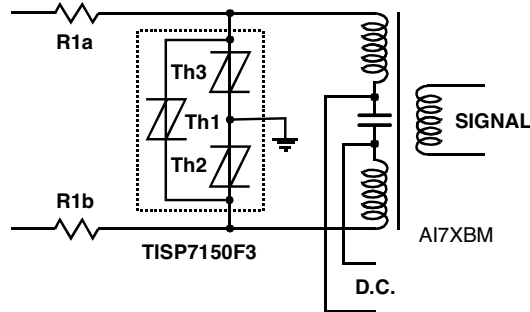
Figure 37. ISDN Protection
