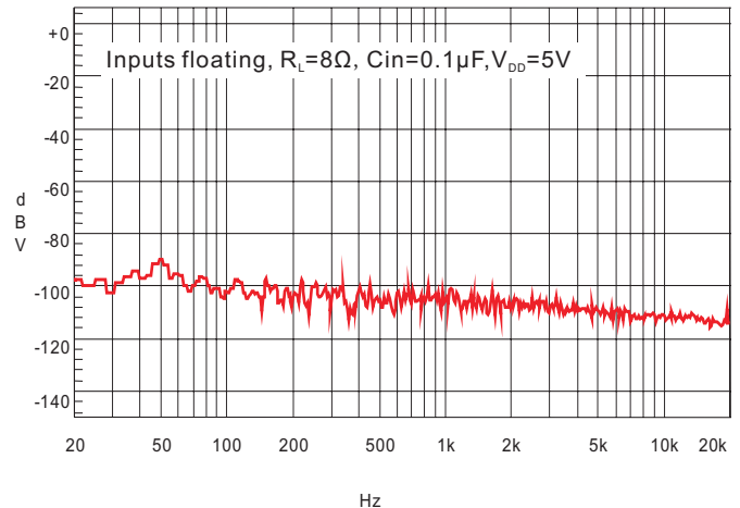
12. Noise Floor
