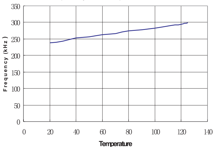
2. Frequency VS Temperature
