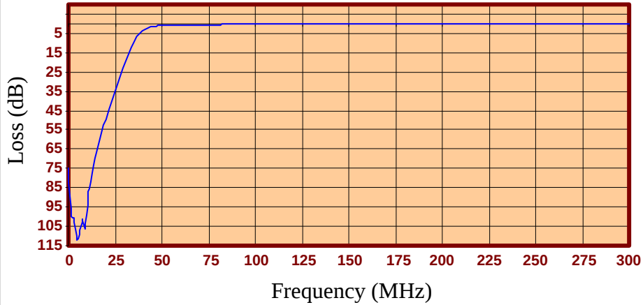
Insertion Loss
