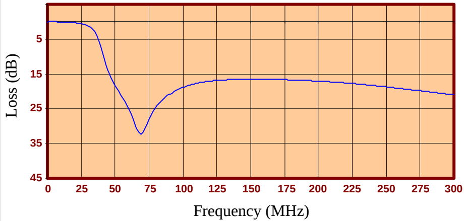
Return Loss
