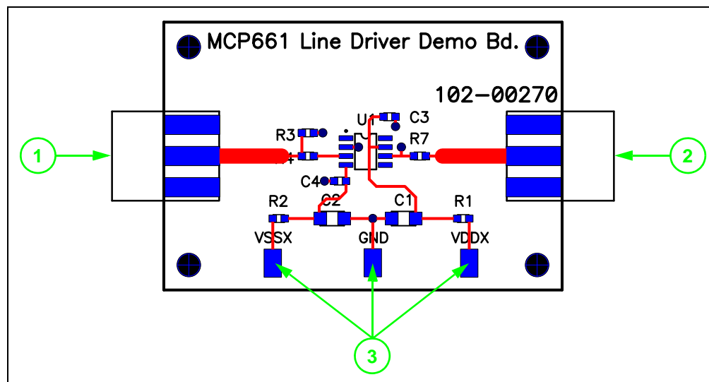
FIGURE 2-1: Lab Equipment Connections.
