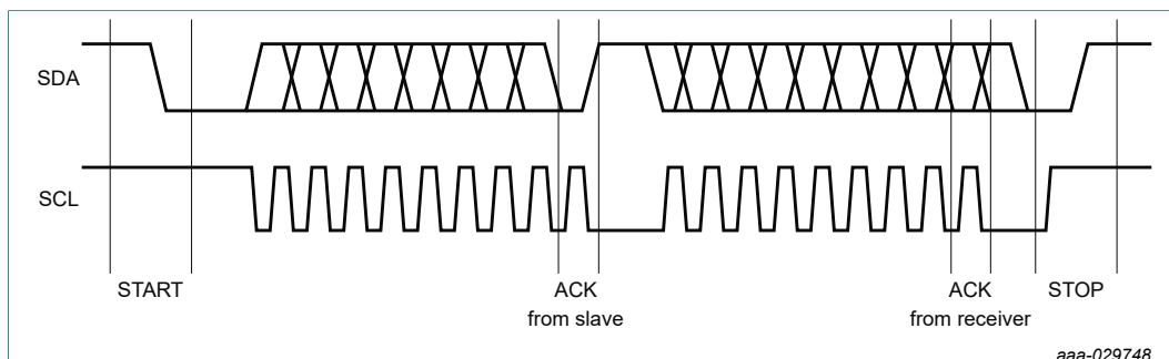
Figure 16. I²C byte transmissions
