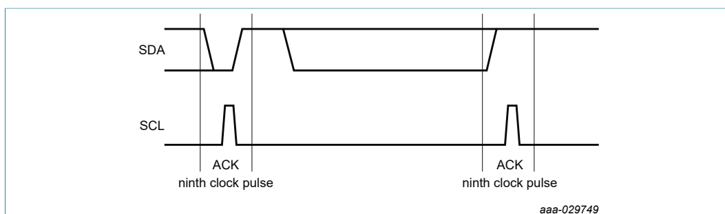
Figure 17. I²C acknowledge and not acknowledge transmission
