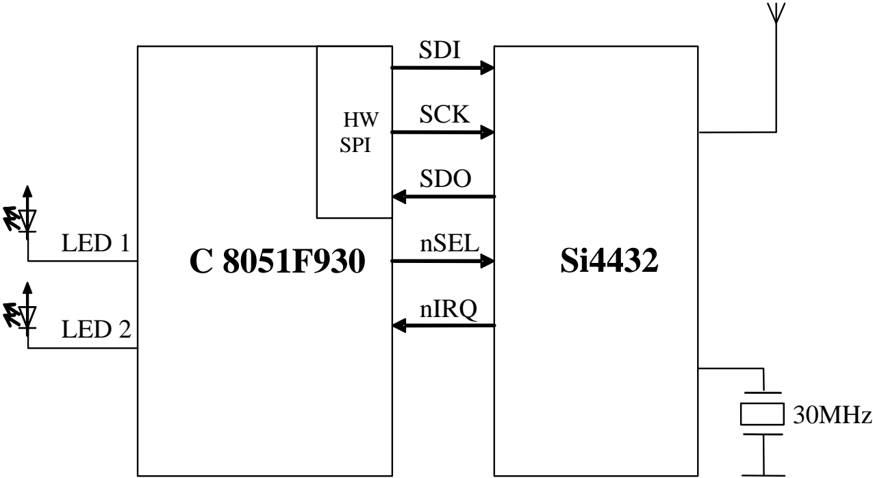
Figure 62. Basic Hardware Connections
