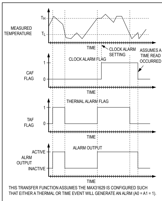
Figure 2. Alarm Transfer Function
