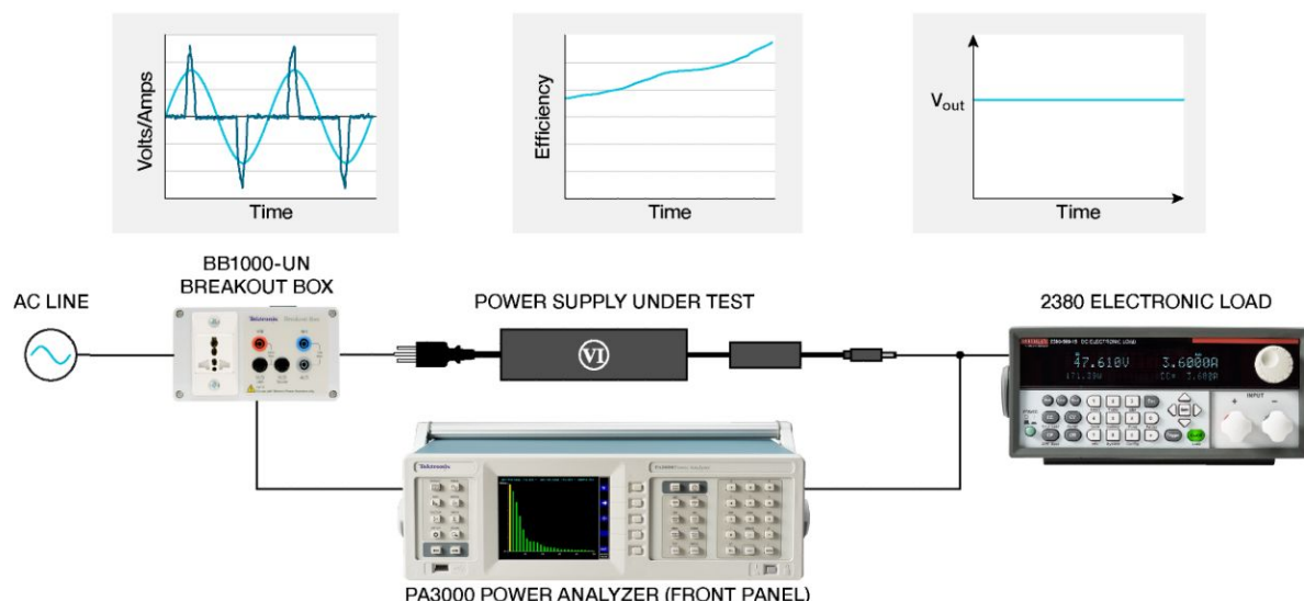
Example test configuration and measurement results for testing AC/DC power supplies and LED drivers
