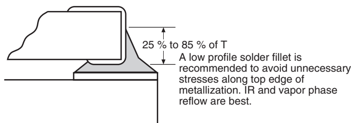
FIGURE 4 - RECOMMENDED MOUNTING (1)(2)(3)
