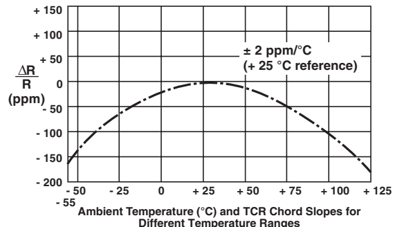
FIGURE 3 - TYPICAL RESISTANCE/TEMPERATURE CURVE
