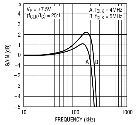
Passband Gain vs f_{CLK} at 85°C
