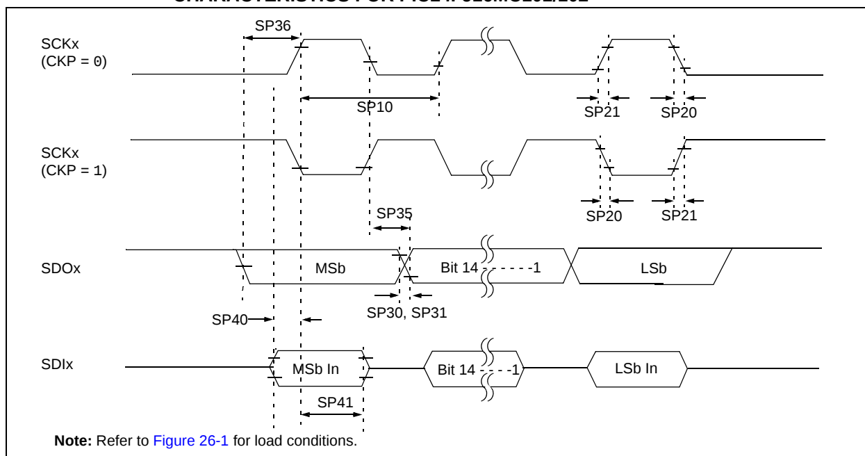
FIGURE 26-13: SPIx MASTER MODE (FULL-DUPLEX, CKP = 1, CKP = X, SMP = 1) TIMING CHARACTERISTICS FOR PIC24FJ16MC101/102
